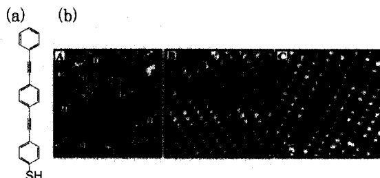
그림 6. (b) Au(111) 표면에 형성된 4-[4'-(phenylethynyl)-phenylethynyl]-benzenethiol (a) self-assembled monolayer를 찍은 STM 사진(A: 300 \text{ \AA} \times 300 \text{ \AA} ), (B와 C: 80 \text{ \AA} \times 80 \text{ \AA} ). Reprint from[18], G. Yang et al., J. Phys. Chem. B, Vol. 104, p. 9059(2000).
